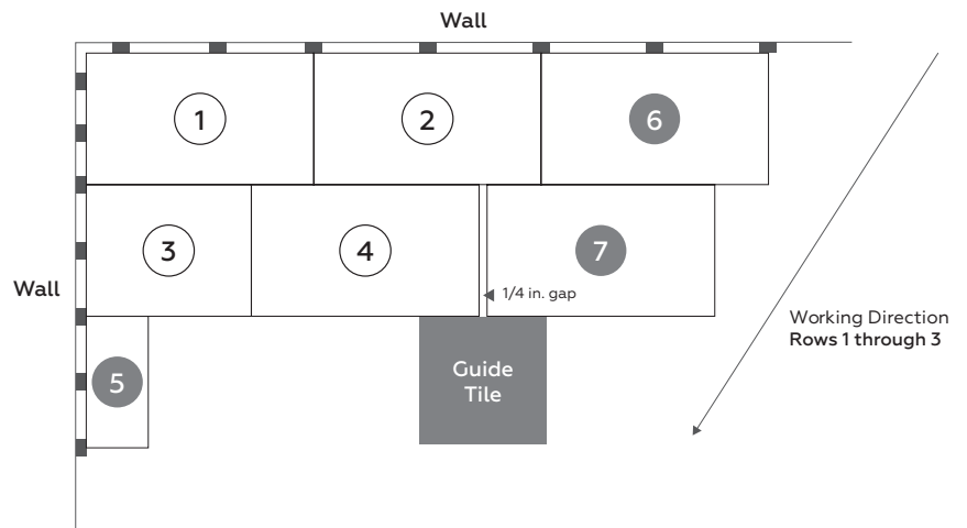
Figure 2: Work in a diagonal pattern for first three rows.
