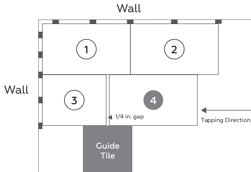
Figure 1: Use guide tile to lock in fourth tile.
